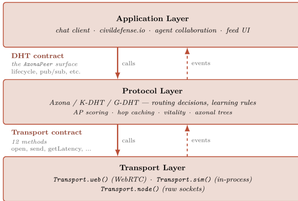
Figure 10. The three-layer architecture. The application layer (chat clients, civildefense.io , agent-collaboration backends) sits above the DHT contract —the AxonaPeer surface, organised into lifecycle, pub/sub, direct-messaging, mesh-introspection, and telemetry clusters. Below the DHT contract lives the protocol layer : the routing decisions and learning rules—Axona, or K-DHT, or G-DHT. Below that is the Transport contract , a twelve-method surface that the network has to provide. Concrete Transports plug in underneath: simTransport() for the in-browser lab, webTransport() for WebRTC in real browsers, nodeTransport.server() for headless servers. Calls travel downward; events travel upward. Neither contract permits the layers on either side to know what the other is doing internally.
